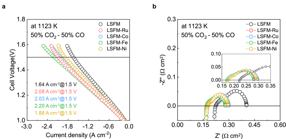
Fig. 4 (a) The \text{CO}_2 electrolysis performance with the infiltrated LSFM electrode feeding \text{CO}_2 : \text{CO} (50:50) at 1123 K. (b) Total impedance spectra of the cell with the infiltrated LSFM electrode at 1123 K.
