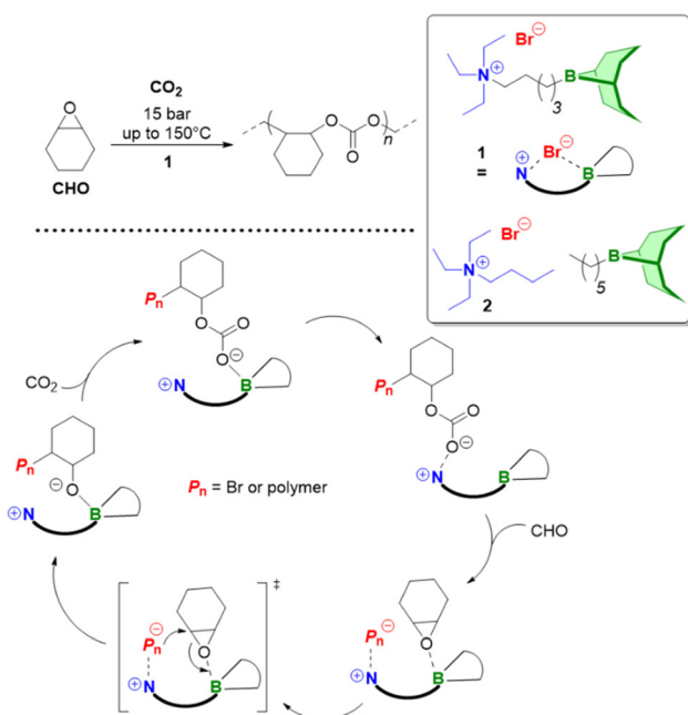
Scheme 18 Polycarbonate formation from \text{CO}_2 and CHO using a bifunctional monoborane as described by Wu.
