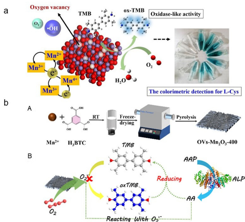
Fig. 6 (a) OVs modulation Mn 3 O 4 nanozyme with enhanced OXD-mimicking performance for L-cysteine detection. Adapted with permission from ref. 101. Copyrights 2021, Elsevier. (b) Preparation of OV-Mn 2 O 3 -400 (A) and the colorimetric sensor for ALP detection (B). Adapted with permission from ref. 102 Copyrights 2023, ACS.
