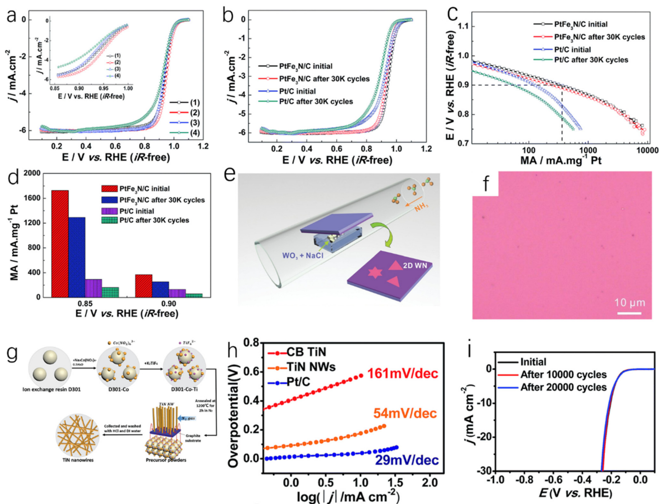
Fig. 4 (a) ORR polarization curve of the catalyst in O_2 -saturated 0.1 mol L^{-1} HClO_4 aqueous solution (25 °C, scanning rate 5 mV s^{-1} , rotation speed 1600 rpm), (inset: high-magnification polarization curve); (b) ORR polarization curves of PtFe_3N/C and Pt/C catalysts before and after ADT in O_2 -saturated 0.1 mol L^{-1} HClO_4 aqueous solution (25 °C, scan rate of 5 mV s^{-1} , rotation speed of 1600 rpm); (c) comparison of mass activity (MA) before and after cycling; (d) comparison of mass activity of PtFe_3N/C and Pt/C before and after cycling at 0.90 V and 0.85 V. 28 Copyright 2015, Royal Society of Chemistry; (e) a schematic CVD synthesis of ultrathin WN; (f) optical image of the product grown on SiO_2/Si substrate (without salt). 31 Copyright 2019, Wiley-VCH; (g) synthetic route of TiN NWs; (h) Tafel plots of TiN NW, CB TiN and Pt/C electrodes; (i) the stability test of TiN NWs catalyst carried out by potential cycling, which shows the initial polarization curve and the polarization curve after 10 000 and 20 000 potential cycles. 32 Copyright 2016, Royal Society of Chemistry.
