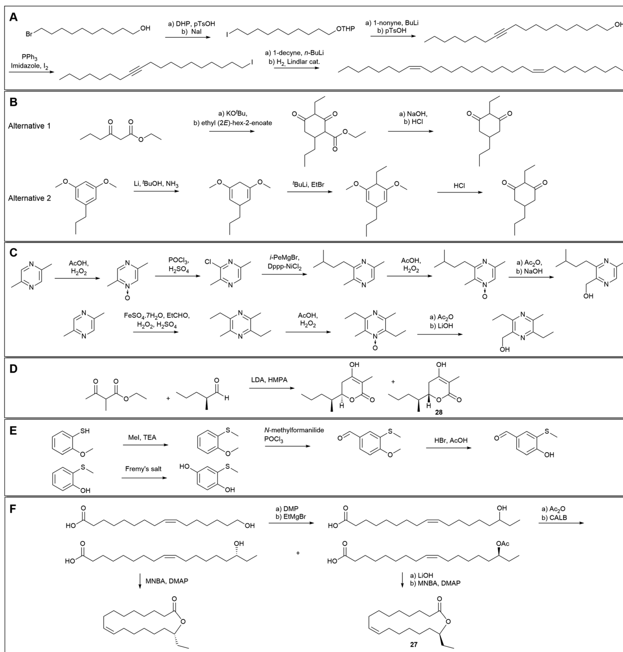
Scheme 1 Examples of synthetic routes to orchid pollinator attractants: (A) (8Z,20Z)-nonacosadiene from Ophrys exaltata , (B). chiloglottone from Chiloglottis spp., (C). hydroxymethylpyrazines from Drakaea livida , (D). drakolide ( 28 ) from Drakaea micrantha , (E). (methylthio)phenols from Caladenia crebra , (F). disalactone ( 27 ) from Disa forficaria .
