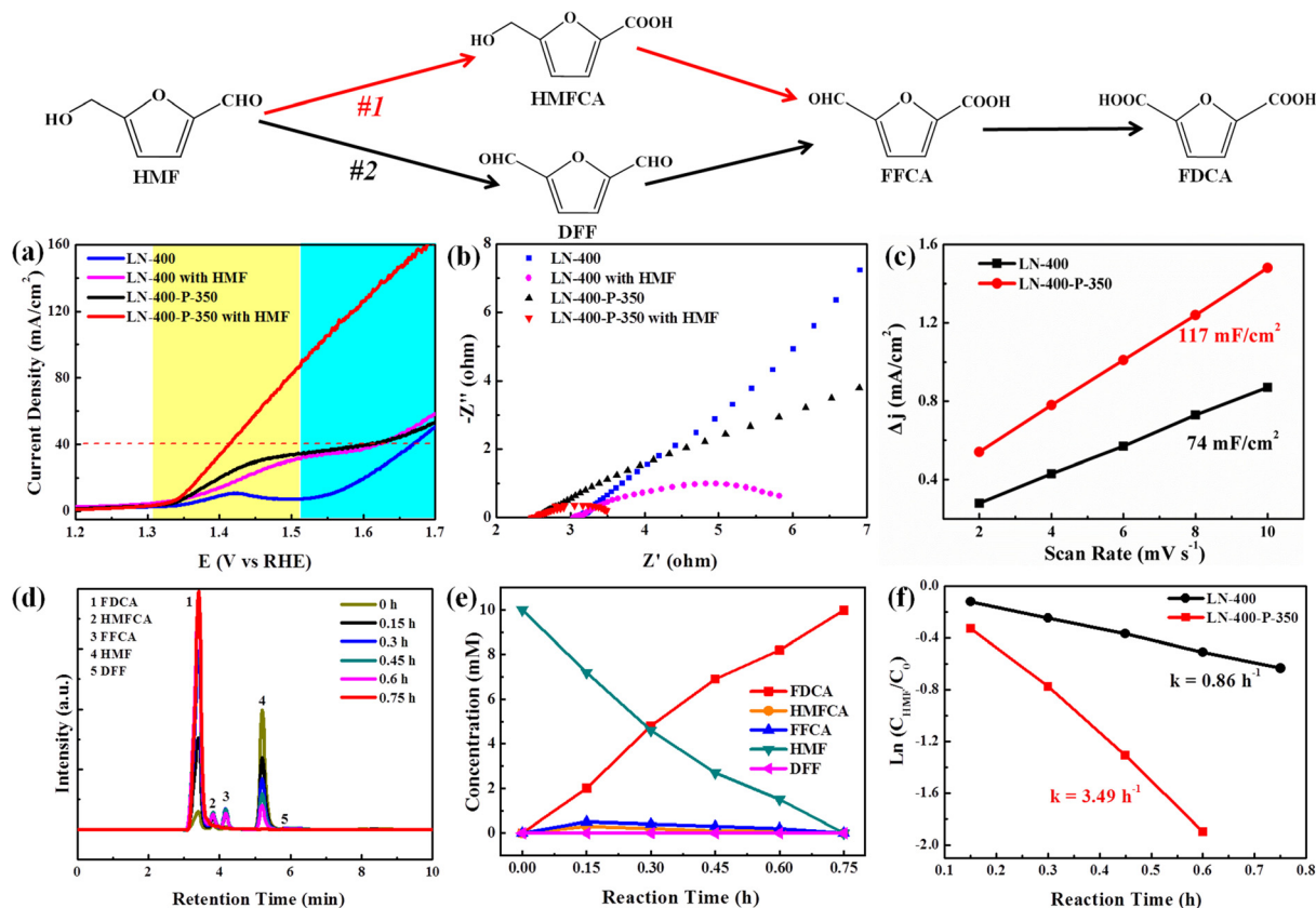
Fig. 3 (a) LSV curves of LN-400 and LN-400-P-350 in 1.0 M KOH without and with 10 mM HMF; (b) Nyquist plots of LN-400 and LN-400-P-350 in 1.0 M KOH; (c) C_{\text{dl}} of LN-400 and LN-400-P-350 in 1.0 M KOH; (d) HPLC chromatograms of ECO of HMF by LN-400-P-350 at 1.49 V vs. RHE in a 1.0 M KOH solution containing 10 mM HMF at various time; (e) concentrations of HMF and the oxidation products at different reaction times in 1.0 M KOH solution containing 10 mM HMF at 1.49 V vs. RHE and (f) kinetic fitting curves of the ECO of HMF by LN-400 and LN-400-P-350.
