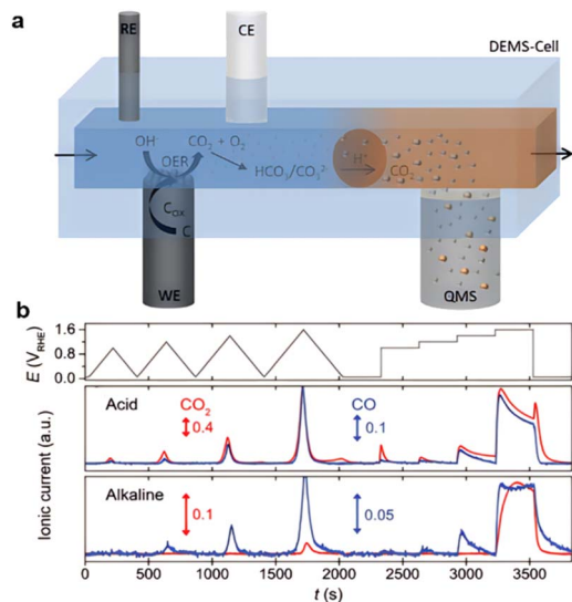
Fig. 6 Observation of high corrosion of carbon during oxidation: (a) DEMSs system, (reproduced from ref. 124 with permission. Copyright © 2020 Wiley-VCH) (b) ionic peak of CO. (Reproduced from ref. 125 with permission from the Royal Society of Chemistry).
