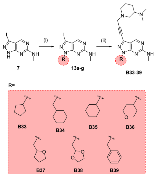
Scheme 6 Synthesis of B33–39 . Reagents and conditions: (i) alkyl bromide, NaH, DMF, 150 °C, \mu\text{W} , 85 min, 24–82%; (ii) 10n , Pd(PPh 3 ) 2 Cl 2 , CuI, TEA, THF, 70 °C, \mu\text{W} , 2 h, 26–44%.
