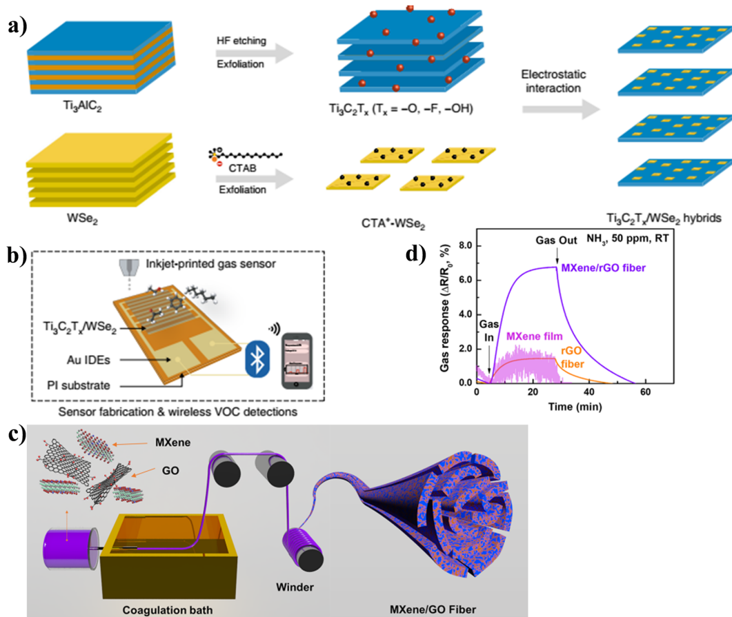
Fig. 9 (a) A schematic representation of the steps involved in the preparation of Ti_3C_2T_x/WSe_2 nanohybrids, (b) illustration of inkjet-printed gas sensors for the detection of VOC using a wireless monitoring system. Reproduced with permission from ref. 102 Copyright 2020. Springer Nature (Open Access), (c) schematic of the spinning process for MXene/GO hybrid fiber, and (d) comparison of the gas response of MXene film, rGO fiber, and MXene/rGO hybrid fiber (40 wt% MXene). Reproduced with permission from ref. 112 Copyright 2020. American Chemical Society.
