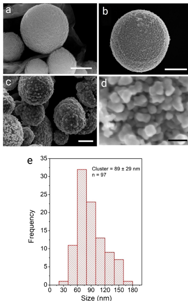
Fig. 1 SEM micrographs of precursor and composite systems prepared using approach 1: (a) o-CμP , (b) CμP-AuNP(DMAP) and (c and d) roughened composites CμP-AuNP-1 . Scale bars show (a–c) 500 nm and (d) 50 nm.
