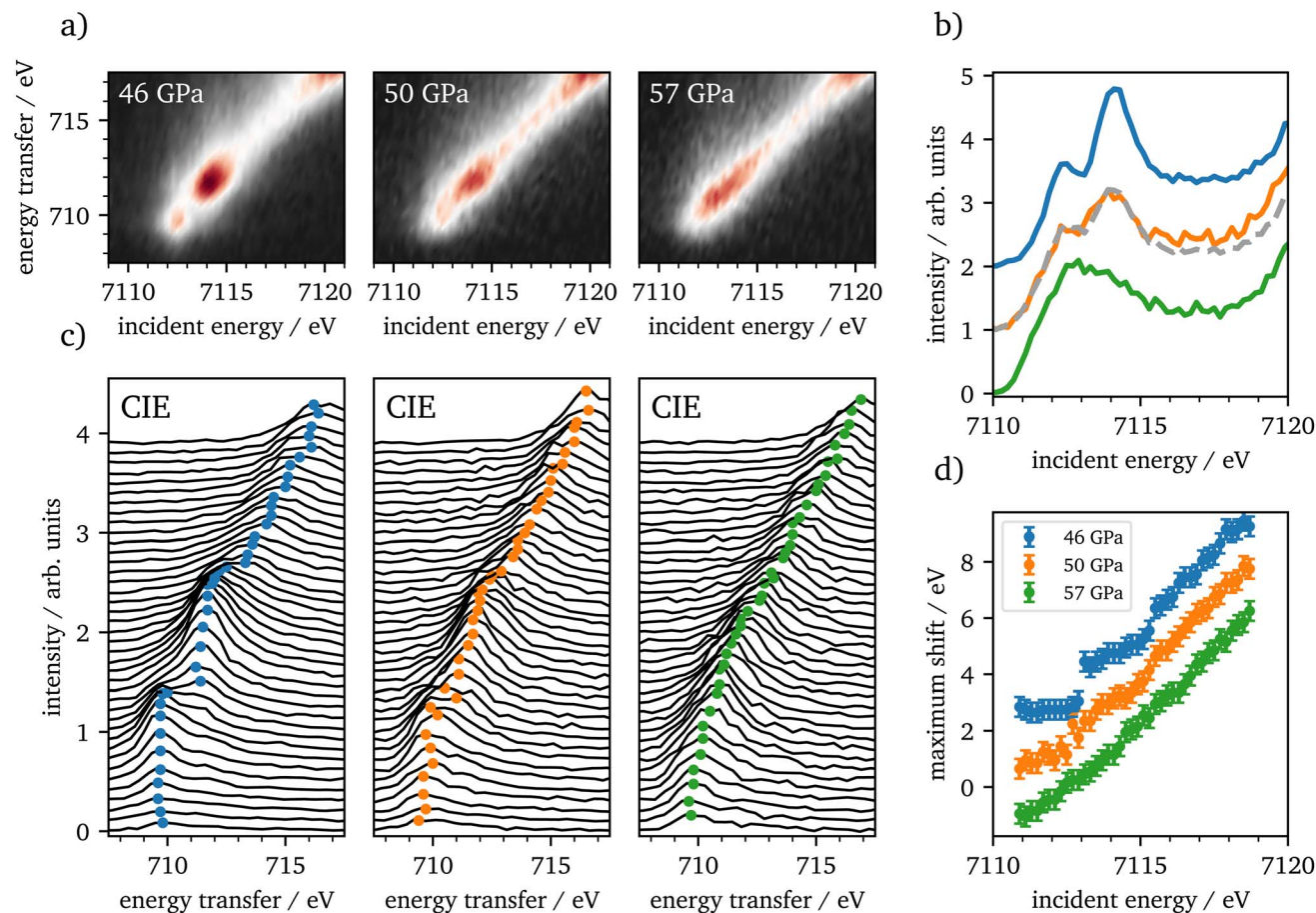
Fig. 6 (a) XRES planes of \text{Fe}_2\text{O}_3 at high pressures of 46 GPa, 50 GPa and 57 GPa. (b) CEE-cuts of the pre-edge region are shown and shifted vertically for clarity. The grey dashed line is a superposition of 46 GPa and 57 GPa with 57% abundance of the HS spectrum. (c) CIE-cuts of each pressure in the pre-edge region, shifted vertically with increasing incident energy. The colored dots indicate the maximum position for each CIE-cut and are visualized in (d), shifted vertically for clarity.
