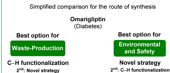
Scheme 17 Summarised assessment for omarigliptin synthesis.
