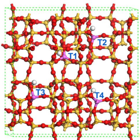
Fig. 9 The optimized periodic structure of HZSM-5 (atomic ratio \text{Si}/\text{Al} \sim 23 , a = 20.615223 \text{ \AA} ; b = 20.430119 \text{ \AA} and c = 13.716548 \text{ \AA} , \alpha = 90.0248^\circ ; \beta = 89.76483^\circ ; \gamma = 90.05055^\circ ). Yellow: Si; red: O; purple: Al; white: protons.
