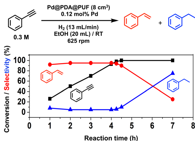
Fig. 5 Hydrogenation of phenylacetylene with Pd@PDA@PUF (8 cm 3 ); EB selectivity. Reaction conditions: PA (6 mmol), Pd (7 × 10 -3 mmol, 0.12 mol%), EtOH (20 mL), H 2 flow rate (13 mL min -1 ), room temperature, 625 rpm.
