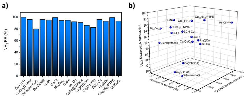
Fig. 1 (a) Previously reported FEs for the \text{NO}_3\text{RR} over selected Cu and Cu-based electrocatalysts. (b) Reported FEs and measured current densities at applied potentials for selected Cu and Cu-based electrocatalysts. Data extracted from ref. 20, 21, 32–36 and 39–47.
