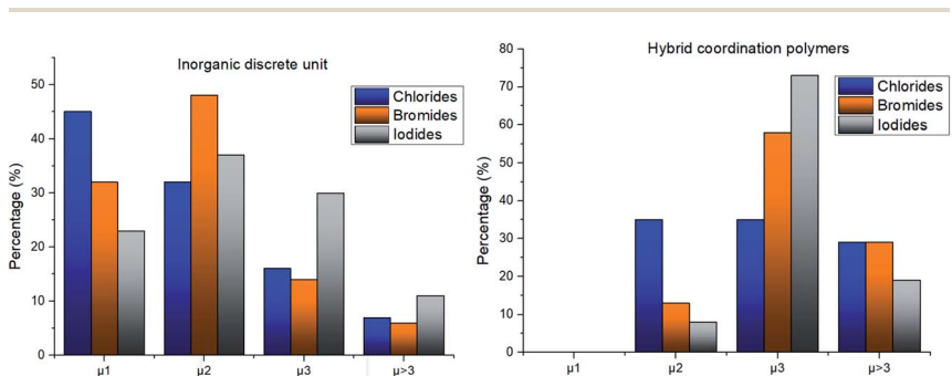
Fig. 2 Percentage of the coordination number of the different halides in the structures that have inorganic discrete units and percentage of the coordination number of the different halides in the hybrid coordination polymers.
