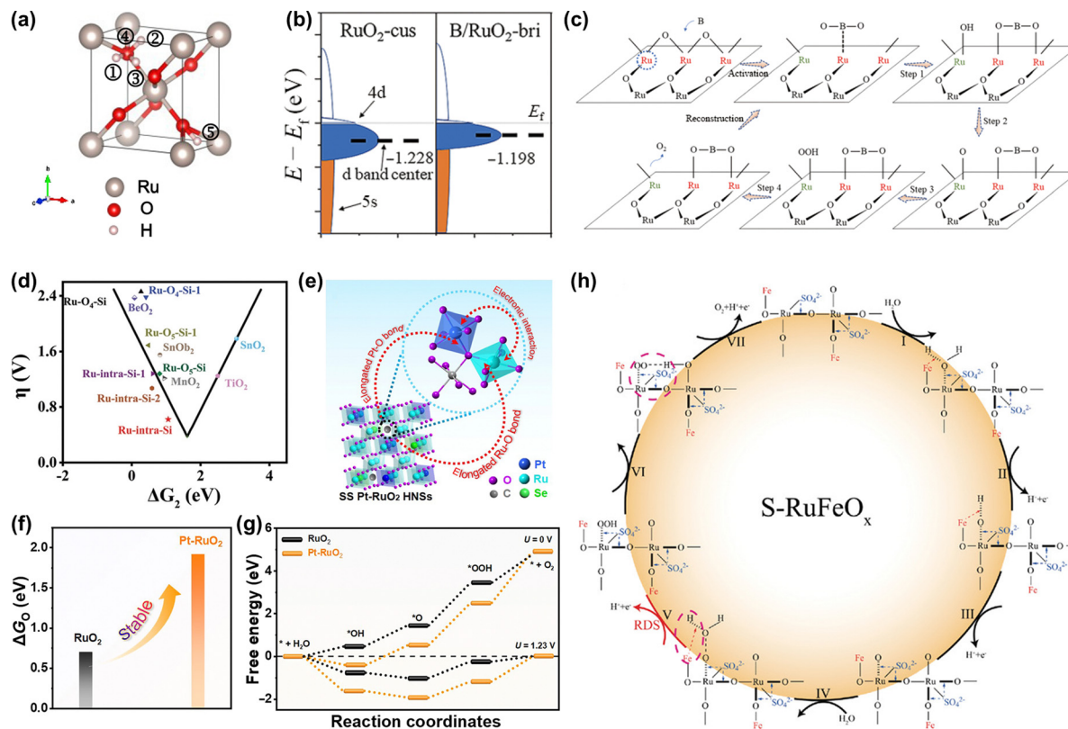
Fig. 13 (a) Structural illustration of proton and electron co-doped \text{RuO}_2 . 147 (b) Schematic diagram of d-band center change of the Ru-bri site of B/RuO 2 . (c) The schematic diagram of BO 2 migration during OER. 149 (d) The calculated overpotential for Si-RuO x @C in the “volcano” plot of overpotential versus \Delta G_2 ( \Delta G_2 = \Delta G_{\text{OH}^*} - \Delta G_{\text{O}^*} ). 152 (e) Structural illustration of SS Pt-RuO 2 HNSs. (f) The calculated dissociation energy of *O in RuO 2 and Pt-RuO 2 , respectively. (g) The free energy profiles of the OER process on RuO 2 and SS Pt-RuO 2 HNSs under the applied overpotential of 0 and 1.23 V (RHE), respectively. 153 (h) Schematic illustration of the reaction mechanism toward acidic OER on S-RuFeO x . 133
