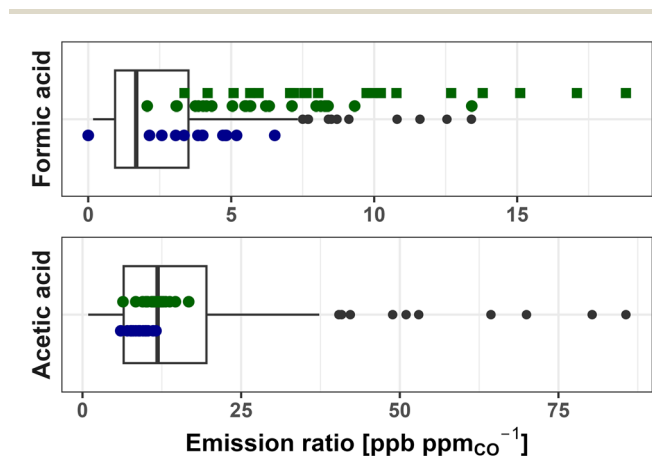
Fig. 2 Emission ratios of formic and acetic acid for literature values (box-and-whisker), WE-CAN PTR-ToF observations (green points), I - CIMS FA (green squares), and FIREX-AQ PTR-ToF (blue points). The box and whisker plots reported include literature ERs from all studies in Table S1,† representing a variety of fuels (204 data points for formic acid and 196 for acetic acid). Boxes represent the 25 th and 75 th percentiles, with vertical lines as median, whiskers as 1.5 \times the interquartile range, and black points as >1.5 \times interquartile range of literature values.
