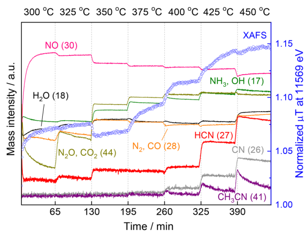
Fig. 4 Changes of the MS spectra and the XAFS intensity (at 11569\text{ eV} ) at various temperatures raising from 300 to 450^\circ\text{C} with 25^\circ\text{C} steps. Reaction conditions: 5 wt% \text{Pt}/\text{Al}_2\text{O}_3 (100 mg), \text{CH}_4:\text{NO}:\text{He} = 13.4:1.8:84.8 (total flow rate: 100\text{ mL min}^{-1} ), and 0.1\text{ MPa} .
