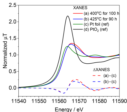
Fig. 3 Pt L_3 -edge XANES spectra of the \text{Pt}/\text{Al}_2\text{O}_3 catalyst after the reaction with methane and nitric oxide at 400^\circ\text{C} for 100 h or 425^\circ\text{C} for 90 h, and the difference XANES spectra of the spent catalysts and Pt foil.
