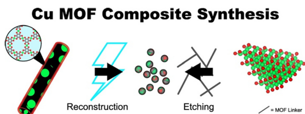
Fig. 22 Representative syntheses for Cu MOF composites. The left-hand side depicts the synthesis of Cu(111) @Cu-THQ via electrochemical reconstruction of Cu-THQ reported by Zhao et al. 146 The right-hand side depicts the synthesis of Cu_2O@Cu-MOF via etching for Cu_2O reported by Tan et al. 128 Green, red, and grey spheres denotes copper, oxygen, and carbon atoms, respectively.
