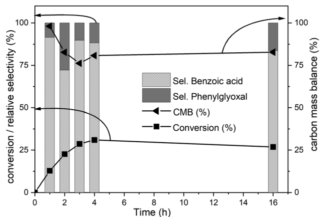
Fig. 3 Time online data for the RICO of biphenyl. Biphenyl conversion (■), carbon mass balance (△), the selectivity of benzoic acid (light grey bars) and selectivity of phenylglyoxal (dark grey bars). The selectivity data reported here are relative selectivity between the two products. Reaction condition: biphenyl: 75 mg; \text{NaO}_4 : 80 mg; \text{RuCl}_3 \cdot x\text{H}_2\text{O} stock solution: 0.23 mL; 2:1 acetonitrile–deionised water solvent mixture: 30 mL; temperature: 22 °C and atmospheric pressure. Molar ratio of substrate : oxidant : catalyst = 1 : 2.67 : 0.03.
