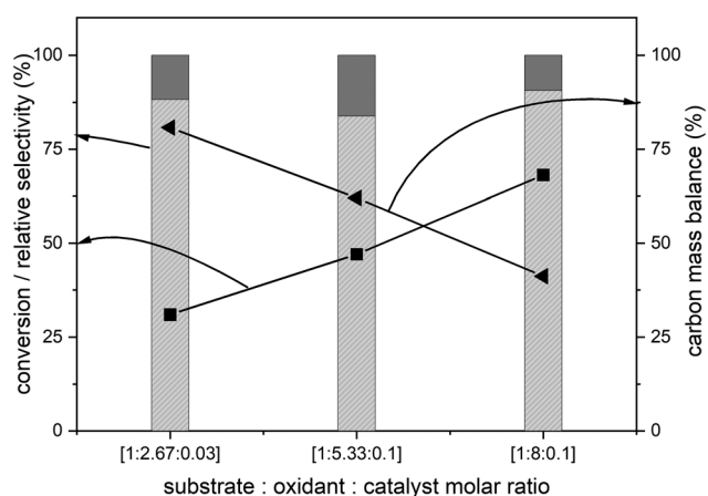
Fig. 4 Effect of the amount of oxidant during the RICO of biphenyl. Biphenyl conversion (■), carbon mass balance (△), the selectivity of benzoic acid (light grey bars) and selectivity of phenylglyoxal (dark grey bars). The selectivity data reported here are relative selectivity between the two products. Reaction condition: biphenyl: 75 mg; \text{NaO}_4 : 80 mg; \text{RuCl}_3 \cdot x\text{H}_2\text{O} stock solution: 0.23 mL; 2:1 acetonitrile–deionised water solvent mixture: 30 mL; temperature: 22 °C and atmospheric pressure.
