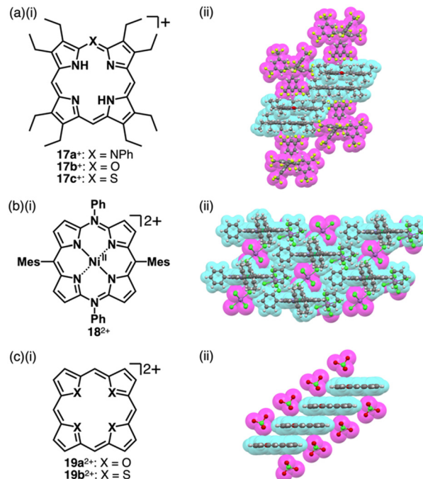
Fig. 10 (a) (i) Heteroatom-containing porphyrins 17a-c + and (ii) single-crystal X-ray structure of 17a + - \text{BARF}^- , (b) (i) tetraaryl-5,15-diazaporphyrin Ni II complex 18 2+ and (ii) single-crystal X-ray structure of 18 2+ - 2\text{SbCl}_6^- and (c) (i) core-modified porphyrins 19a,b 2+ and (ii) single-crystal X-ray structure of 19a 2+ - 2\text{ClO}_4^- . The crystal structures are redrawn from cif files: 2033992, 1437728 and 1166405. Atom colour codes in (b) (c) (ii) and the following figures: green, blue-green and purple in the ball-and-stick models refer to chlorine, nickel and antimony, respectively.
