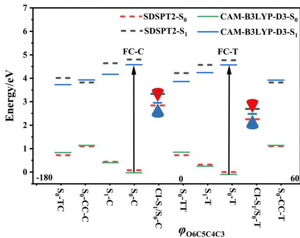
Fig. 3 Potential energy profiles for DPC isomers; the eight minima plus two conical intersections with respect to the \varphi_{\text{O6C5C4C3}} dihedral angle. FC-C and FC-T stand for the Franck–Condon regions for its corresponding S_0 -C and S_0 -T minima, respectively. The SDSPT2 energy calculations (dashed lines) were carried out at (TD)-CAM-B3LYP-D3 optimized geometries (solid lines).
