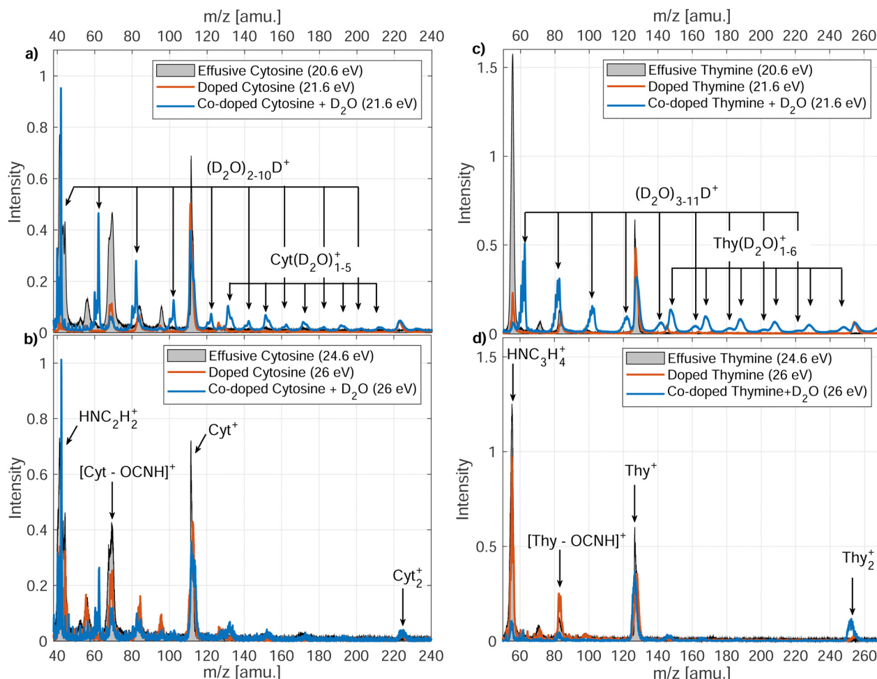
Fig. 3 Mass spectra recorded for Cyt [(a) and (b)] and Thy [(c) and (d)] in an effusive molecular beam, doped into HNDs or co-doped with D 2 O into HNDs. (a) and (c) show the mass spectra for Penning ionization of the dopant ( h\nu = 21.6 eV), and (b) and (d) show mass spectra for charge-transfer ionization ( h\nu = 26 eV). In case of photoionization of the effusive beam, the photon energy is matched to the internal energy of the excited He atom inducing Penning ionization and to the He ion inducing charge-transfer ionization.
