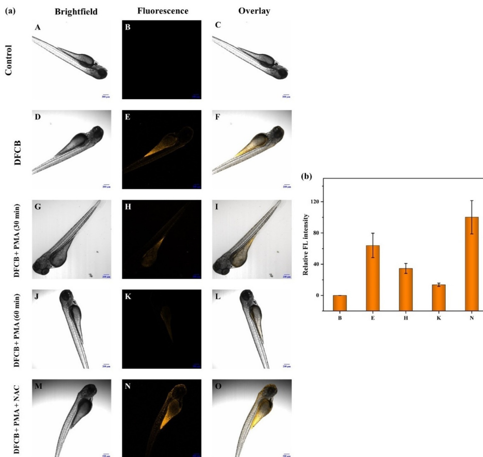
Fig. 11 (a) The imaging of \text{H}_2\text{O}_2 in zebrafish: (A–C) zebrafish alone were cultured for 1 h; (D–F) zebrafish supplemented with the DFCB sensor ( 4\ \mu\text{M} ) were cultured for 1 h; (G–I) zebrafish supplemented with PMA ( 1\ \mu\text{g}\ \text{mL}^{-1} ) were cultured for 30 min; (J–L) subsequently, the zebrafish supplemented with PMA ( 1\ \mu\text{g}\ \text{mL}^{-1} ) were cultured for 60 min; and (M–O) the zebrafish were cultured with PMA ( 1\ \mu\text{g}\ \text{mL}^{-1} ) and then incubated with NAC ( 1\ \text{mM} ), followed by staining with the DFCB sensor ( 4\ \mu\text{M} ) for 1 h. (b) Quantitative intensity obtained from fluorescent images of zebrafish.
