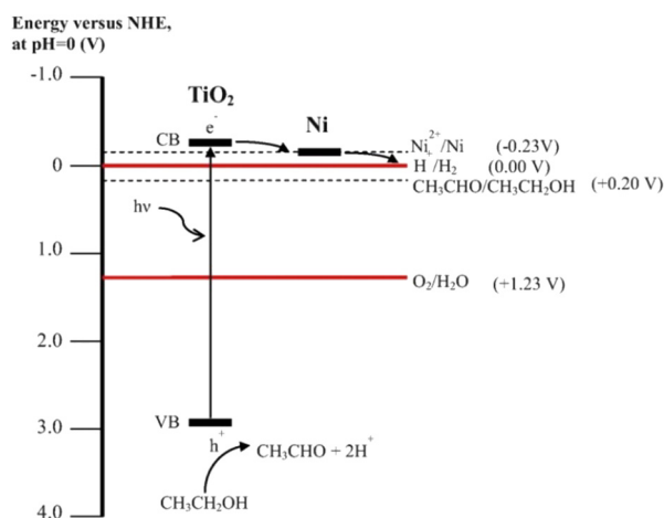
Fig. 20 Schematic illustration of important electron transfer processes in the Ni/ \text{TiO}_2 system leading to \text{H}_2 production. Reprinted with permission from Elsevier. 231
