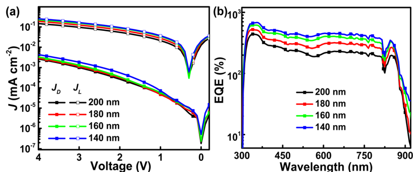
Fig. 2 (a) J - V curves and (b) EQE spectra under 4 V applied bias of PM-APDs.
