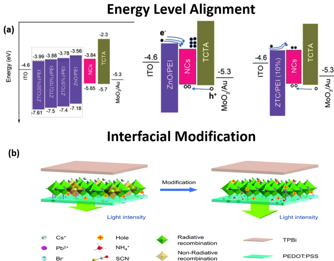
Fig. 7 (a) Device energy-level diagram for MXene modified transfer layer in the PeLEDs (left) and charge carrier injection and recombination mechanisms for 0% (middle), and 10% (right) MXenes based devices. ZTC in the diagram represents \text{ZnO-Ti}_2\text{C}_2 . Reproduced with permission from ref. 150. Copyright © 2020 The Authors. Published by Wiley-VCH GmbH; (b) schematic illustration of the interface defect passivation mechanism of perovskite films via ammonium thiocyanate modification. Reproduced with permission from ref. 155. Copyright © 2021, The Royal Society of Chemistry.
