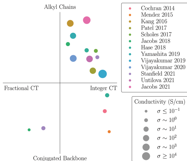
Fig. 2 Compilation of available experimental data for PBTBT and P3HT, relating the position of molecular dopants in the polymer lamellae (alkyl chains vs. conjugated backbone) to the nature of the host–dopant complexes (integer vs. fractional CT). The electrical conductivities of each sample is expressed through the size of the marker, see legend. The position of different points in each quadrant is arbitrary. We note that the large majority of doped polythiophenes feature integer CT, except for two systems corresponding to dopants inserted in the conjugated backbones. The systems with the largest conductivities are characterized by dopants inserted in the alkyl region and integer CT (upper-right quadrant).
