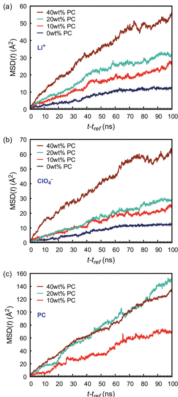
Fig. 7 Mean square deviations in the z-direction for (a) \text{Li}^+ , (b) \text{ClO}_4^- and (c) PC at different PC weight ratios.
