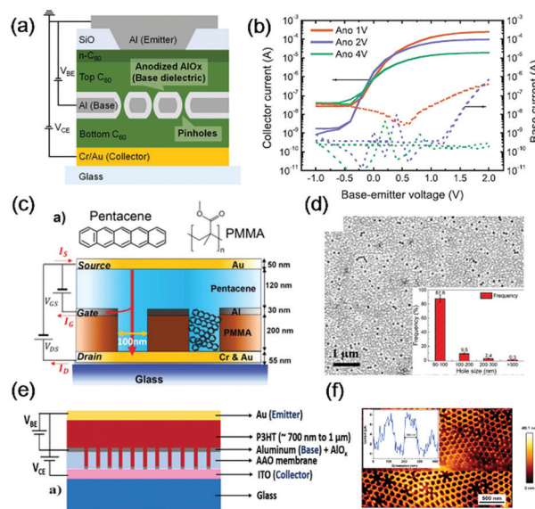
Fig. 4 (a) Device scheme of a SCLVTs with an electrochemically oxidized permeable base electrode and (b) transfer curves of these SCLVTs under an emitter–collector voltage V_{\text{CE}} of 1 V. Anod 1 V, 2 V and 4 V represent the different anodized Al base electrodes with anodizing potentials of 1, 2, and 4 V. 37 Copyright 2019, Wiley-VCH. (c) Cross-section scheme of the built-in channels in SCLVTs developed by Guo et al. (d) Al surface in these devices after removing spheres. The inset shows the size distribution of the nanoholes left on the Al film. 36 Copyright 2020, Wiley-VCH. (e) Device structure of SCLVTs based on mesoporous alumina templates. (f) AFM image of the porous anodized alumina membranes. 39 Copyright 2017, American Chemical Society.
