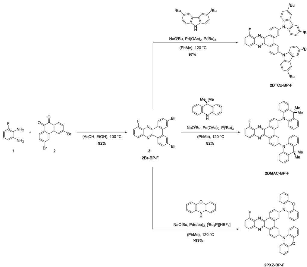
Scheme 1 Synthesis of 2DTCz-BP-F , 2DMAC-BP-F , and 2PXZ-BP-F .
