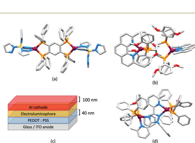
Fig. 22 Structures of (a) [Cu 2 (pz 4 B) 2 (μ-tpbz)] (CSD refcode KURCAD), and (b) the cationic complex in [Cu 2 (2,9-Me 2 phen) 2 (μ-MeOdpccb)][PF 6 ] 2 (refcode VOZQAE). (c) Architecture of a LEC containing [Cu 2 (2,9-Me 2 phen) 2 (μ-MeOdpccb)][PF 6 ] 2 in the active layer; the LEC was driven under a bias of 4 or 5 V. (d) Structure of the dinuclear cation in [Cu 2 (POP) 2 (μ- 37 )] 2 [BF 4 ] 2 (refcode MAMXUW). H atoms are omitted from the figures for clarity.
