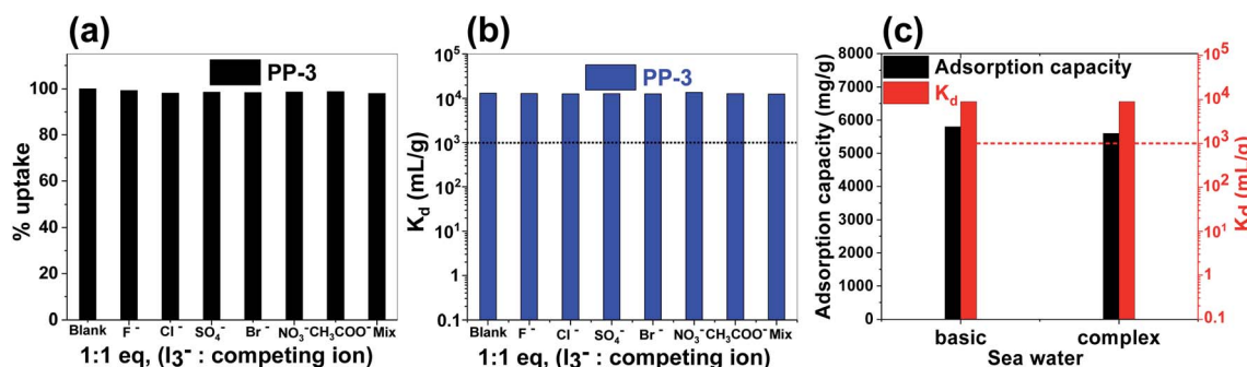
Fig. 7 (a) Uptake percent for I_3^- anions in the presence of other competing anions, (b) distribution coefficient ( K_d ) graph and (c) I_3^- adsorption capacity from the basic and complex seawater and the corresponding distribution coefficient value ( K_d ).
