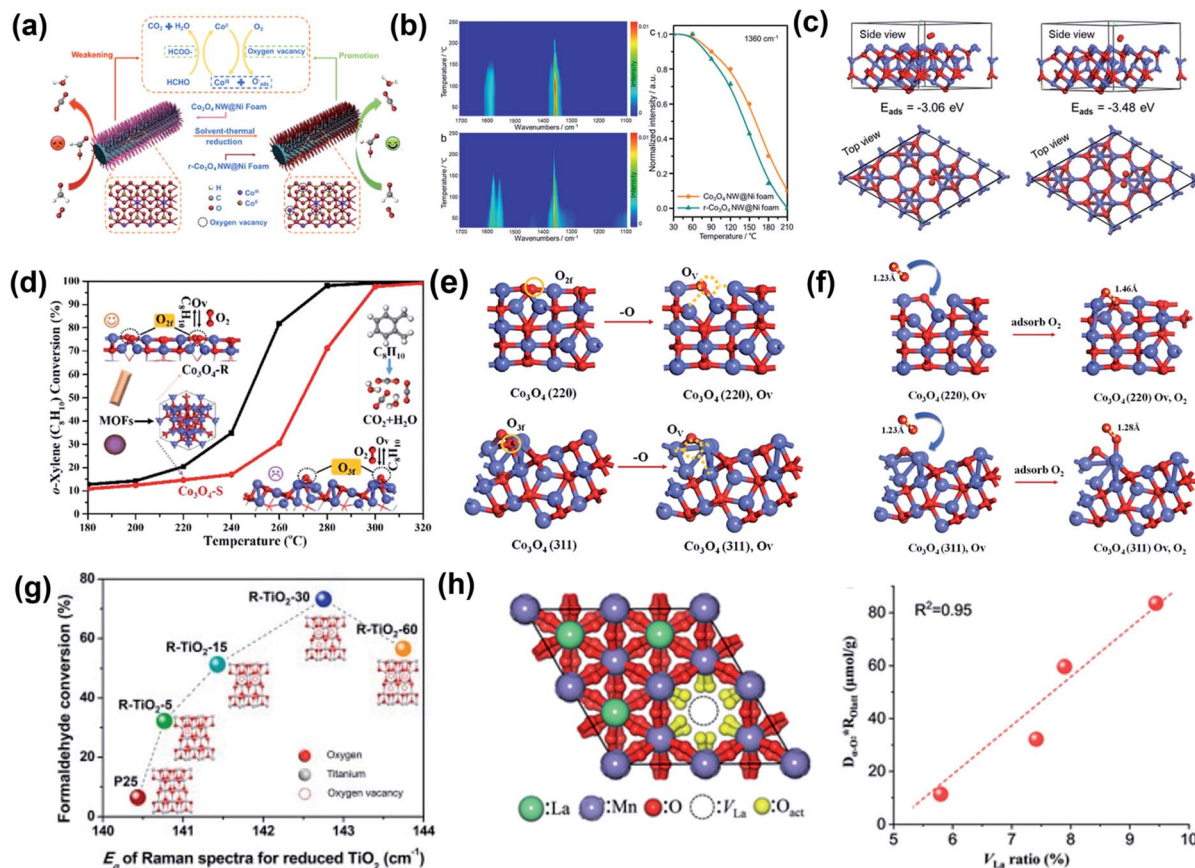
Fig. 21 (a) Schematic illustration of the catalytic oxidation of HCHO over r-Co 3 O 4 NW@Ni with OV; (b) In situ DRIFTS after HCHO adsorption over Co 3 O 4 NW@Ni and r-Co 3 O 4 NW@Ni catalysts as a function of temperature. (c) O 2 molecule adsorbed on the (111) surface of Co 3 O 4 NW@Ni foam and r-Co 3 O 4 NW@Ni catalysts. Adapted with permission from ref. 293 Copyright (2020) American Chemical Society. (d) Catalytic oxidation activities of o-xylene over MOF-derived Co 3 O 4 with different shapes. (e) OV formation over the (220) and (311) surfaces of Co 3 O 4 , respectively; (f) side view of the adsorption configuration of O 2 over the (220) and (311) surfaces of Co 3 O 4 with OV. The Co and O atoms are in blue and red, respectively. Adapted with permission from ref. 294 Copyright (2021) American Chemical Society. (g) Formaldehyde conversion over reduced TiO 2 of different OV concentrations. Adapted with permission from ref. 296 Copyright (2019) Elsevier. (h) Activation of surface lattice oxygen induced by La vacancies and the amount of released surface O latt (D α-O 2 RO latt ) as a function of V La ratio. Adapted with permission from ref. 297 Copyright (2021) Wiley-VCH Verlag GmbH & Co. KGaA.
