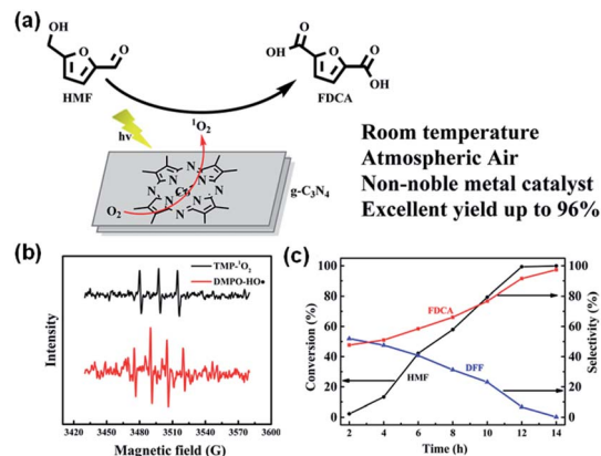
Fig. 20 (a) Possible mechanism of the photocatalytic oxidation of HMF with the CoPz/g-C 3 N 4 catalyst. (b) EPR signals of the DMPO·HO· adduct in water in the presence of bulk g-C 3 N 4 and the TMP- 1 O 2 adduct in water in the presence of CoPz/g-C 3 N 4 in the photocatalysis process. (c) Photocatalytic performance. Adapted with permission from ref. 287 Copyright (2017) American Chemical Society.
