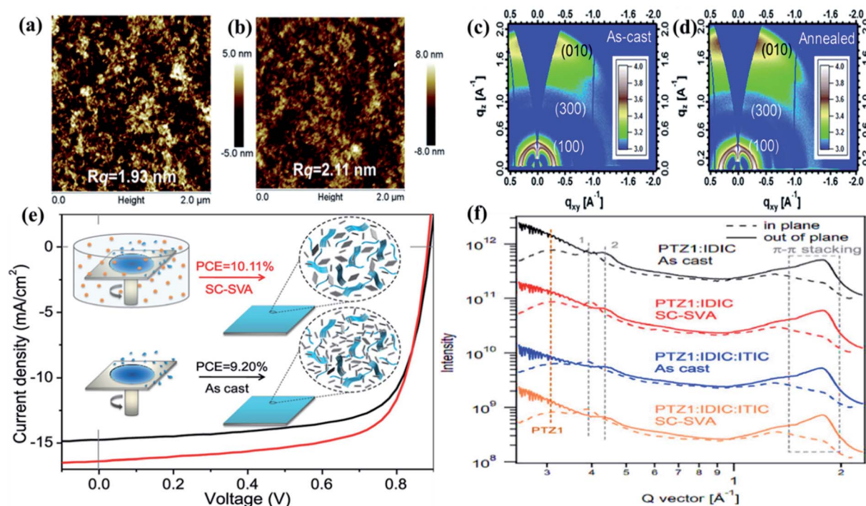
Fig. 13 Tapping-mode AFM topography of PBDB-T/IT-M thick-film devices: (a) after annealing and (b) as-cast films; (c and d) 2D GIWAXS patterns of as-cast and annealed PBDB-T/IT-M thick-films (~250 nm). Reproduced with permission. 198 Copyright 2019, Royal Society of Chemistry. (e) J–V characteristics of PTB7-Th:ITIC devices with or without SC-SVA. (inset: diagram of PTB7-Th:ITIC blends produced with various process). (f) GIWAXS line profiles of PTZ1:IDIC and PTZ1:IDIC:ITIC blend films with or without SC-SVA. Reproduced with permission. 202 Copyright 2017, Elsevier Science Publishers.
