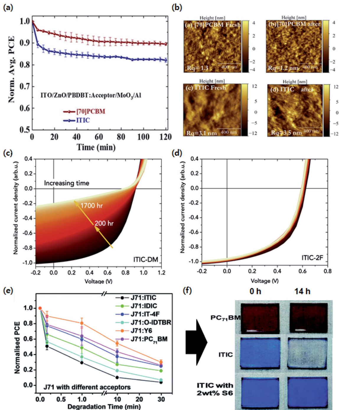
Fig. 21 (a) Performance of PBDB-T-based inverted OSCs under continuous illumination. (b) AFM images of fresh and exposed organic thin films (PC 71 BM and ITIC). Reprinted with permission. 268 Copyright (2019) American Chemical Society. Device stability under continuous illumination in a dry nitrogen atmosphere. Normalised J - V curves of representative devices based on (c) ITIC-DM and (d) ITIC-2F under continuous LED illumination. Reproduced with permission. 270 Copyright (2019) Elsevier. (e) Normalised PCE of J71 devices based on degraded BHJ blends as a function of illumination time. (f) Photographs of photo-oxidised PC 71 BM, ITIC, and ITIC with 2 wt% S6 films as a function of the exposure time. Reproduced with permission. 272 The Royal Society of Chemistry.
