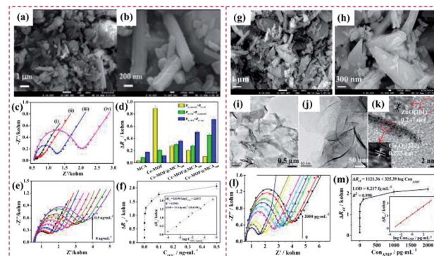
Fig. 27 (a) and (b) SEM images of Ce-MOF@MCA 500 nanohybrids. (c) EIS Nyquist plots of the OTC detection procedures using the electrochemical aptasensors based on Ce-MOF@MCA 500 in 5 mM [Fe(CN) 6 ] 3-/4- containing 0.1 M KCl. (d) Corresponding variations in the R_{ct} values of the five types of aptasensors for detecting OTC. (e) EIS Nyquist plots for the detection of different concentrations of OTC using the Ce-MOF@MCA 500 -based aptasensor. (f) Corresponding calibration curves between \Delta R_{ct} and OTC concentrations (inset: the linear fit plot of \Delta R_{ct} as a function of the logarithm of OTC concentration). Reproduced from ref. 95 with permission from Elsevier, Copyright 2019. (g) and (h) Low- and high-magnification FE-SEM images of Co-MOF@TPN-COF. (i, j, and k) TEM and HR-TEM images of Co-MOF@TPN-COF. (l) EIS responses of the Co-MOF@TPN-COF-based aptasensor with different AMP concentrations. (m) Dependence of \Delta R_{ct} on the concentration of AMP. The linear parts of the calibration curves are shown in the inset of (l). Reproduced from ref. 94 with permission from Elsevier, Copyright 2019.
