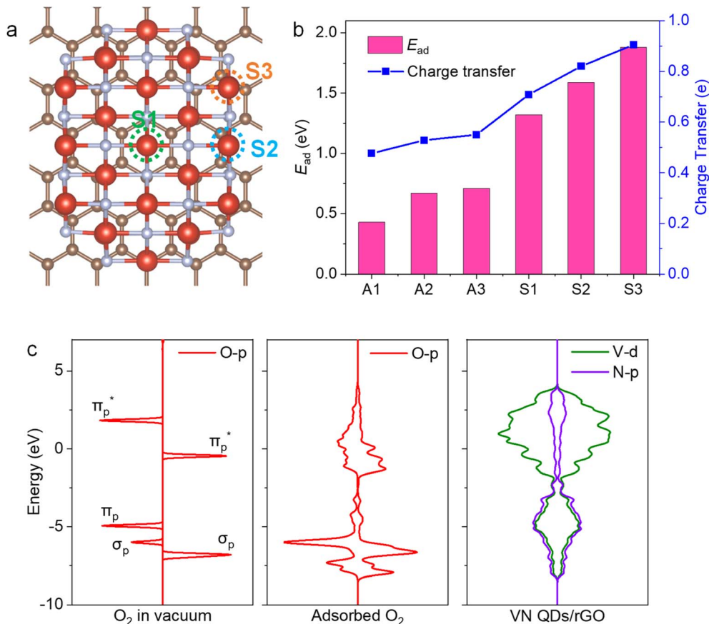
Fig. 4 Investigation of the catalytic mechanism by DFT calculations. (a) Top view of the schematic structure for the four-atom-thick VN QD on a graphene sheet. (b) Adsorption energies and numbers of charge transfer for O 2 adsorbed on different sites. (c) PDOS results of O 2 in a vacuum, adsorbed O 2 and VN QDs/rGO.
