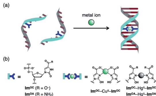
Fig. 1 (a) Schematic diagram of DNA duplexes with a metal-mediated base pair. (b) Molecular structures of novel ligand-type nucleotides bearing 2-oxo-imidazole-4-carboxylate ( Im C ) or 2-oxo-imidazole-4-carboxamide ( Im OA ) as a nucleobase. The expected structures of metal-mediated base pairs are also shown.
