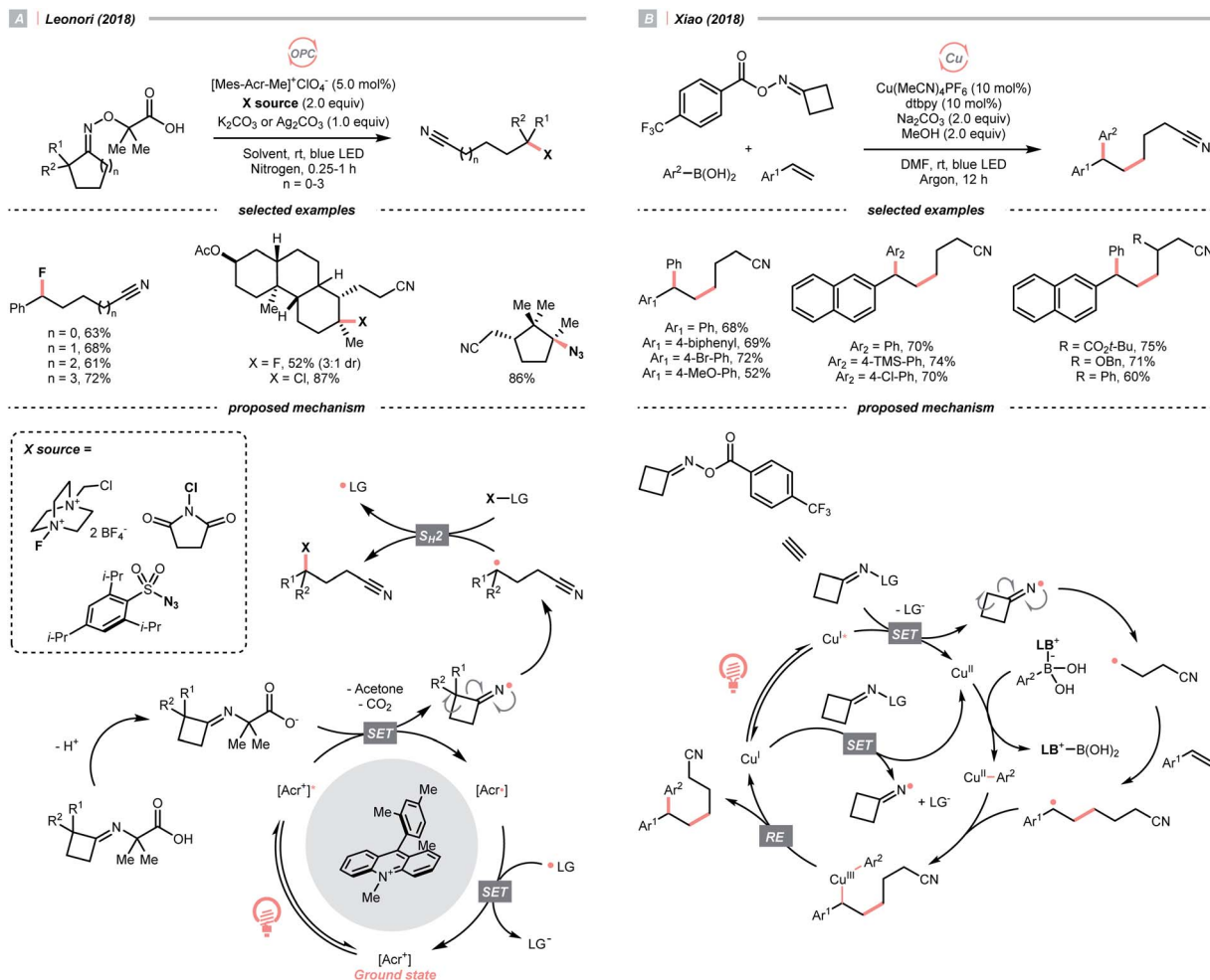
Scheme 26 R^{\bullet} formation via iminyl radical-induced ring-openings.
