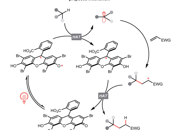
Scheme 11 Eosin Y-catalysed C(sp 3 ) radical generation.
