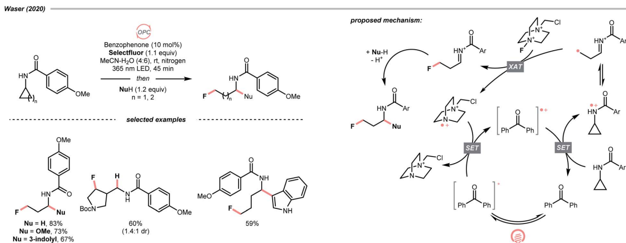
Scheme 27 Generating R^{\bullet} from oxidative ring-opening of amide.
