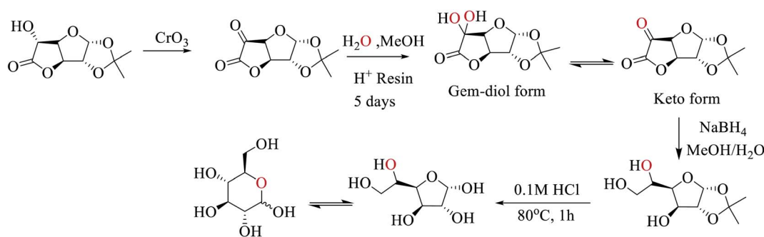
Scheme 2 Three synthetic strategies used in this work to prepare site-specifically ^{17}\text{O} -labeled D-glucose.
