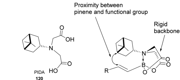
Fig. 11 Pinene-derived iminodiacyclic acid (PIDA).
