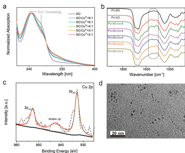
Fig. 1 Structural characterization studies of the PU-SO-Cu elastomer. (a) UV-Vis spectra of samples with different SO : Cu 2+ ratios in MeOH. The curves were normalized using the absorption band at about 250 nm. (b) FT-IR spectra of different samples. (c) The XPS spectrum of the Cu 2p region in PU-SO-Cu. (d) TEM image of a dynamic interaction system in the PU-SO-Cu substrate. Scale bar: 20 nm.
