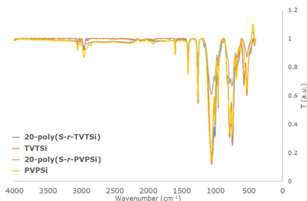
Fig. 1 FTIR spectrum comparison of TVTSi (orange) and 20-poly(S- r -TVTSi) (blue), 20-poly(S- r -PVPSi) (grey) and PVPSi (yellow).
