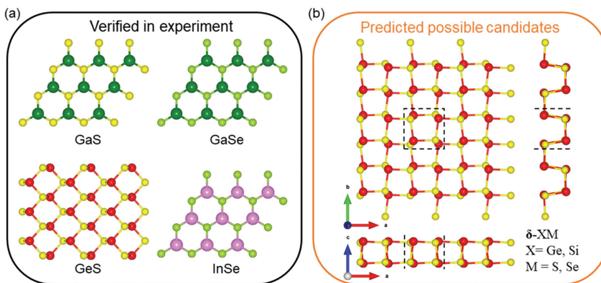
Fig. 1 (a) Synthesized IV–VI monolayers in a previous experiment and (b) crystal structure of the newly predicted \delta -IV–VI monolayers XM ( X = \text{Ge} and \text{Si} ; M = \text{S} and \text{Se} ). The yellow and red balls are M and X atoms, respectively.
