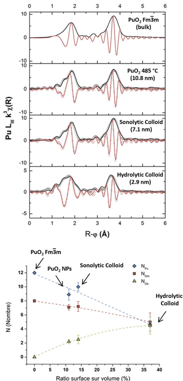
Fig. 15 Top: FT magnitudes of experimental k^3 -weighted EXAFS spectra acquired at the Pu L_3 edge on \text{PuO}_2 nanoparticles in comparison to a reference (black curve, data obtained in the 2–14 \text{\AA}^{-1} range). Bottom: correlation of the coordination numbers obtained for the three Pu–O distances used to fit the Pu–O shell as a function of the S/V ratio of the nanoparticle. Adapted from ref. 96 with permission from Nature Publishing Group, copyright 2017.
