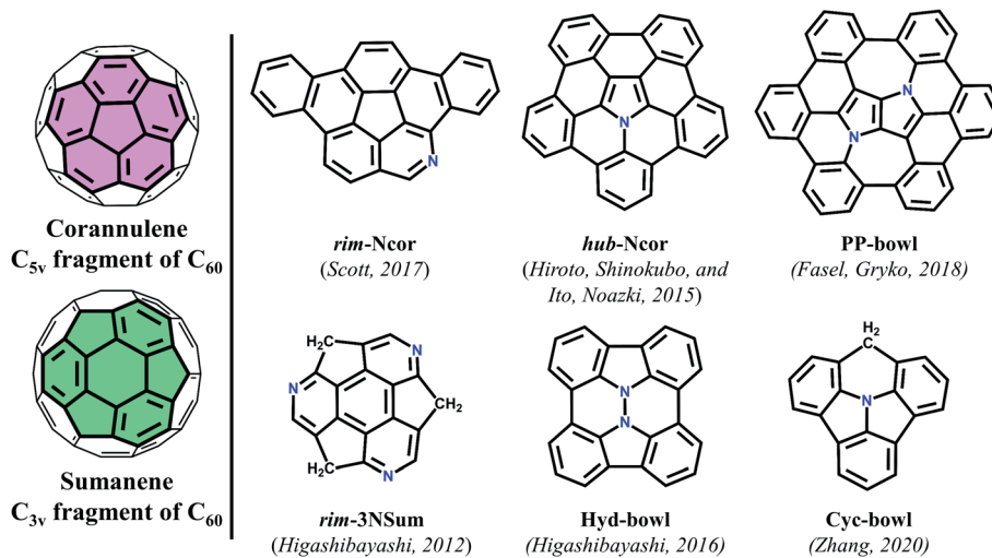
Fig. 1 Structures of nitrogen-containing molecular bowls.
