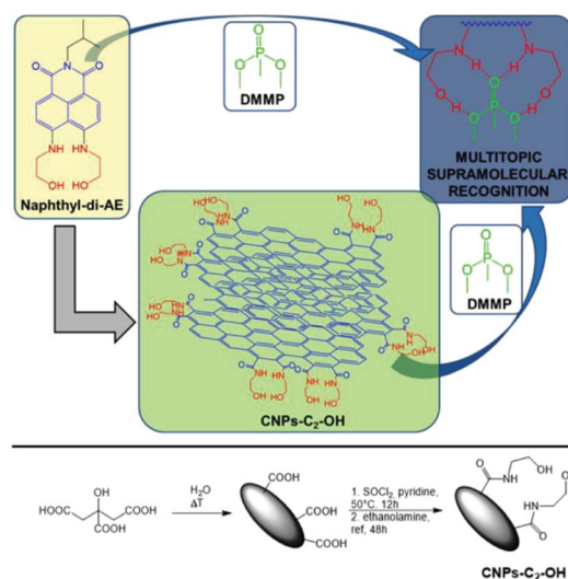
Fig. 11 Representation of \text{CNP-C}_2\text{-OH} and DMMP chelation mechanism. Bottom: Synthesis of \text{CNP-C}_2\text{-OH} (reproduced with permission from ACS Appl. Nano Mater. , 2020, 3, 8182–8191, Copyright 2020, the American Chemical Society).
