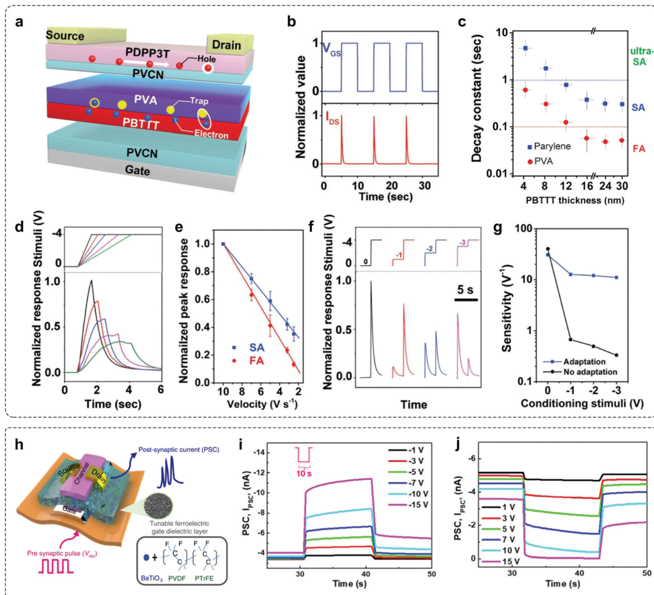
Fig. 7 Examples of adaptive transistors with novel device geometry. (a) Schematic diagram of the proposed organic adaptive device. PBT TT/PVA is buried with the PVCN dielectric layer to facilitate adaptive electron trapping. (b) Time-dependent I_{DS} response upon V_{GS} pulses. The applied V_{DS} and V_{GS} were -1 and -4 V, respectively. (c) Fine-tuned decay constants of ultra-SA, SA, and FA devices as a function of PBT TT film thickness with PVA or parylene dielectrics. (d) Time-dependent response of SA-OATs with different onset speed of stimuli. (e) Peak response of SA- and FA-OATs as a function of onset speed of stimuli. (f) Response of SA-OATs to a periodically increased stimulus. (g) Correlation between sensitivity to the latter stimuli and conditioning stimuli. Reproduced with permission. 30 Copyright 2019, Wiley-VCH. (h) Sketch of the device structure. Gate dielectric layer consists of BT NPs/PVDF-TrFE ferroelectric material. (i and j) Mimicking slowly adapting reception properties of the Fe-OFET. The output current of the device was recorded by applying a sustained potential of -10 V and 10 V with varying amplitude ( \sim 10 s). Reproduced with permission. 14 Copyright 2020, The Author(s).
