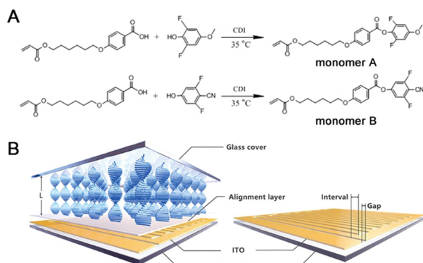
Fig. 1 Synthetic routes of monomer A and monomer B (A); structure diagram of horizontally aligned CLCP coating over the transparent interdigitated comb-shape electrode (conducting layer: indium tin oxide (ITO); gap: 30 \mu\text{m} ; interval: 30, 60 and 120 \mu\text{m} ) (B).
